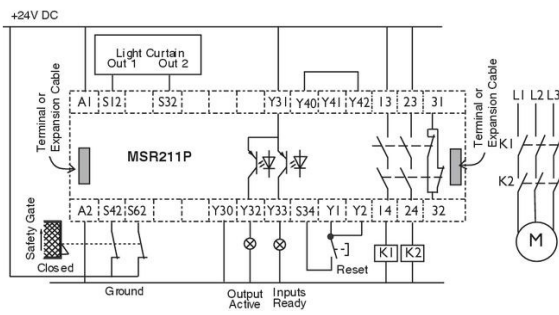
Light Curtain and Dual Channel Safety Gate, Monitored Manual Reset, No Monitored Output
