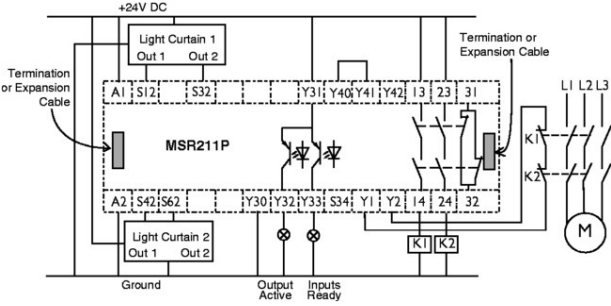
Two Light Curtains, Automatic Reset, Monitored Output
